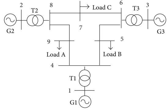
FIGURE 1: One-line diagram of the test network: WSCC 3-machine, 9-bus system [10].
