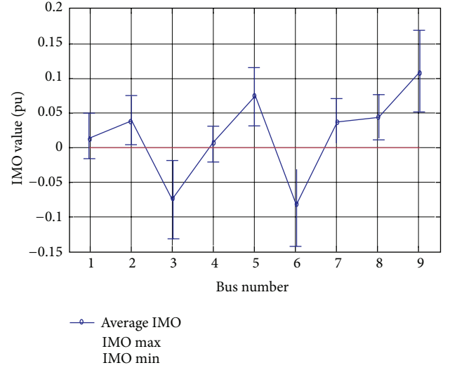
FIGURE 9: IMO values for the 70 MW (LLP = 22.22%) scenario of the Monte Carlo simulation for each bus.
