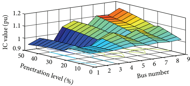
FIGURE 5: Remaining Line Capacity (IC) versus location of RES power plant and load level penetration.
