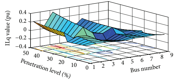
FIGURE 3: Reactive power losses (ILq) versus location of RES power plant and load level penetration.
