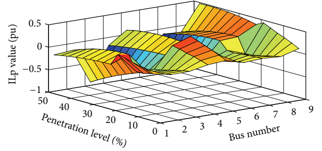
FIGURE 2: Active power losses (ILp) versus location of RES power plant and load level penetration.
