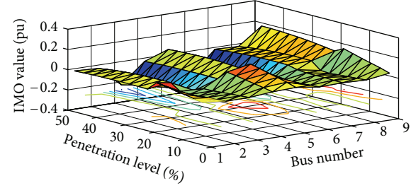
FIGURE 8: Multi-objective assessment (IMO) versus location of RES power plant and load Level penetration utilizing the weight values of Table 5.
