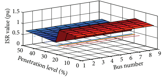
FIGURE 7: Spinning reserve (ISR) versus location of RES power plant and load level penetration.
