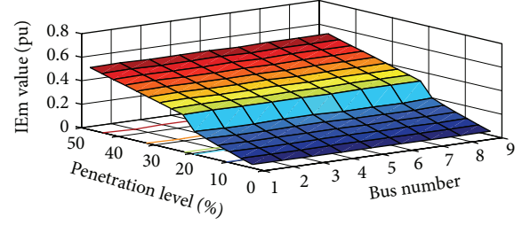
FIGURE 6: Emissions' reduction (IEm) versus location of RES power plant and load level penetration.
