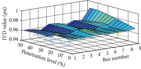
FIGURE 4: Voltage profile (IVD) versus location of RES power plant and load level penetration.
