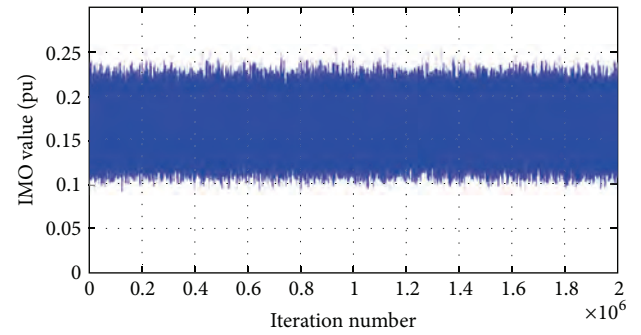
FIGURE 10: IMO values for the best case scenario of the Monte Carlo simulation.
